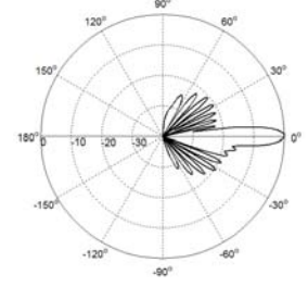
Elevation(High Band)
